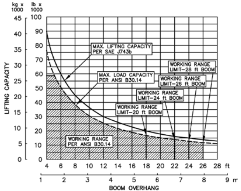
M572c Hydraulic Sideboom Attachment
